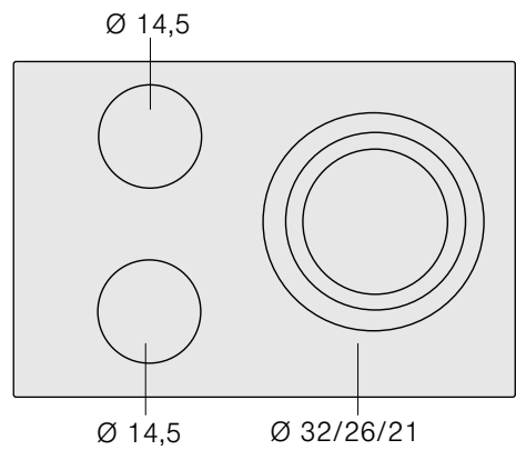
PKD7..FB1.
